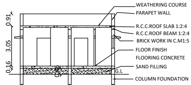
SECTION- SS
