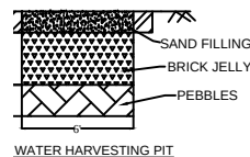
WATER HARVESTING PIT
