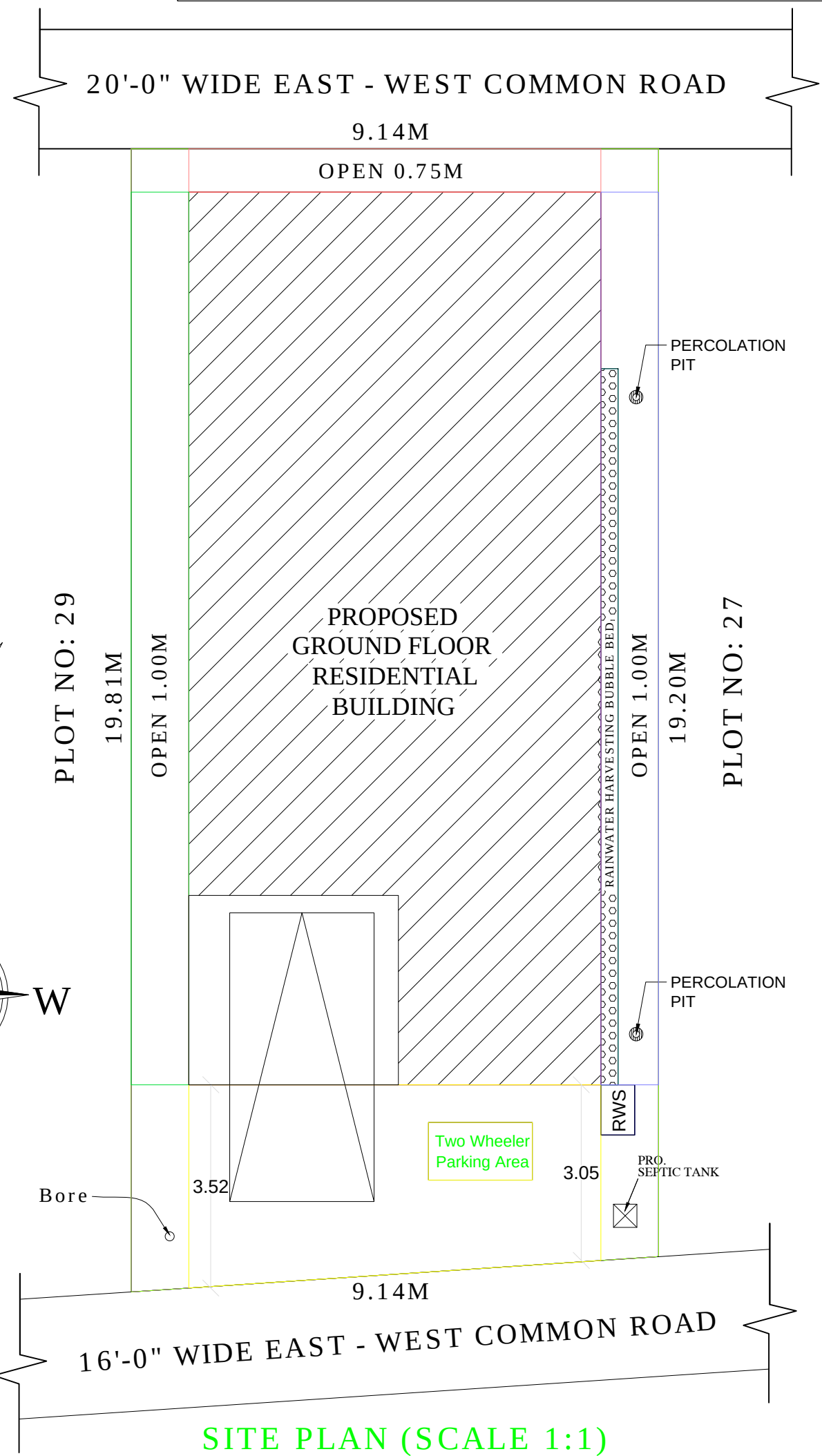
KEY PLAN
