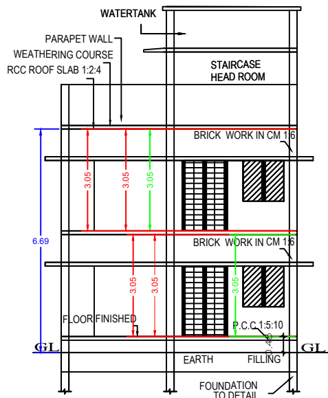
SECTION "A-B"
