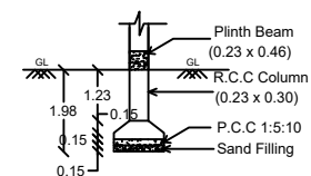
FOUNDATION DETAILS ( Scale 1:100 )
