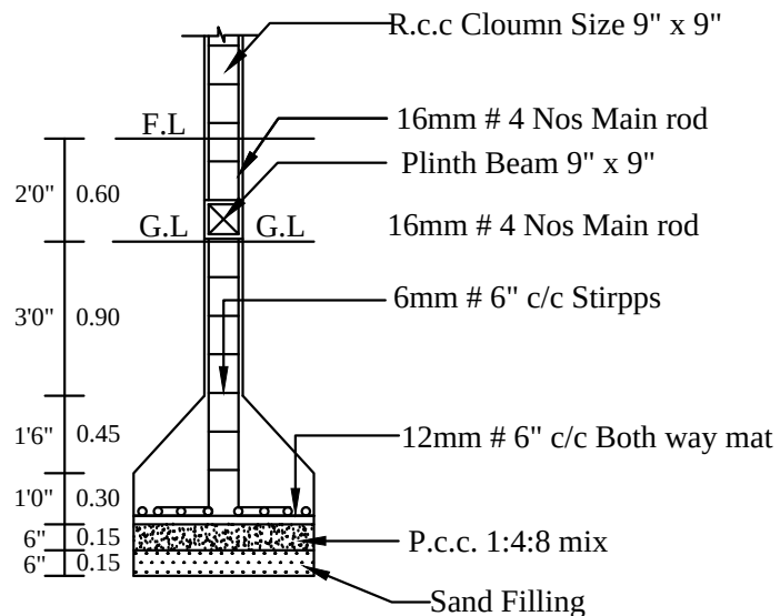
COLUMN DETIAL
