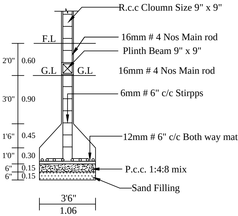
COLUMN DETIALS
