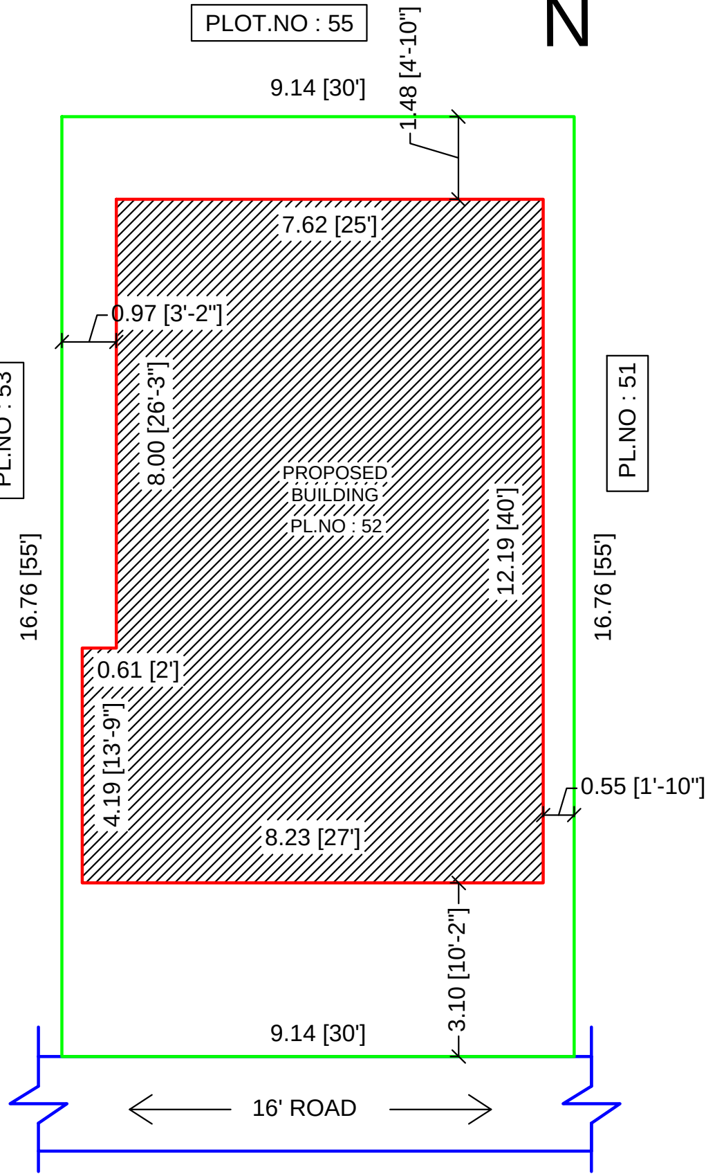
SITE PLAN (1:100)
