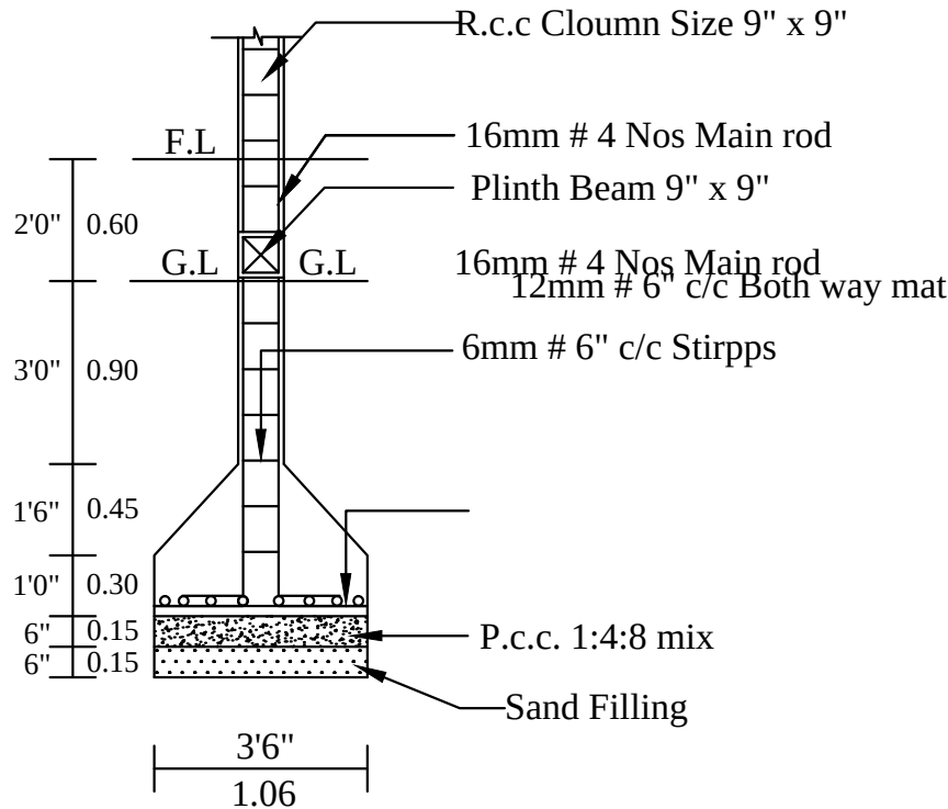
COLUMN DETIAL
