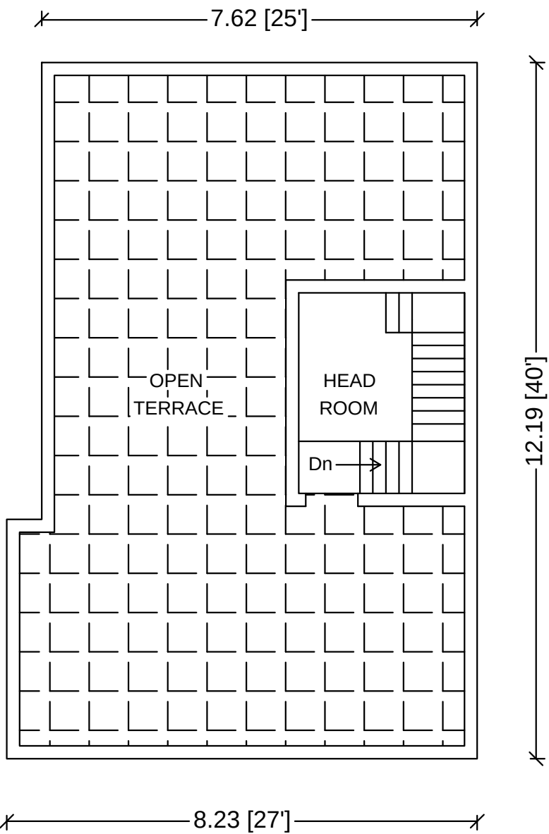
HEAD ROOM PLAN
