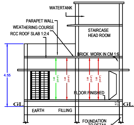
SECTION "A-B"
