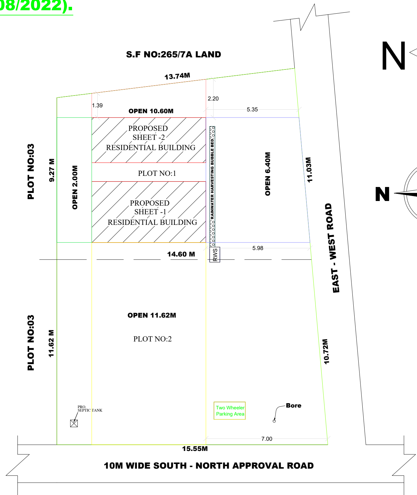
SITE PLAN (SCALE 1:1)
