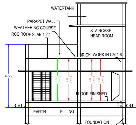
SECTION "A-B"
