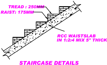
STAIRCASE DETAILS
