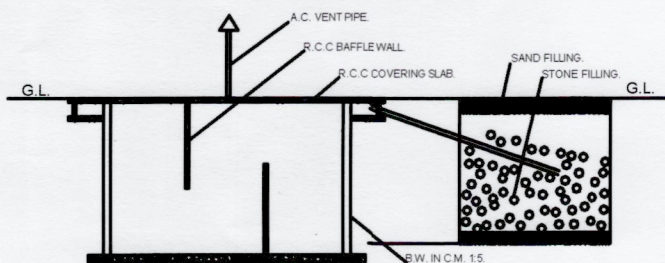
DET - OF SEPTIC TANK & D. TRENCH
