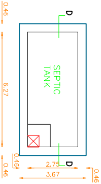
PLAN OF SEPTIC TANK SCALE 1"=20'
