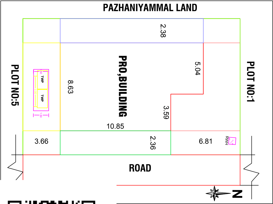
SITE PLAN
