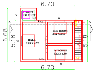
FLOOR- GROUND
