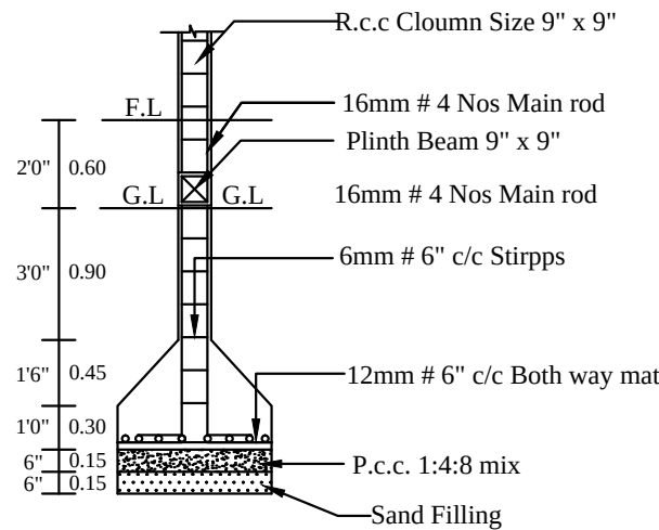
COLUMN DETIAL
