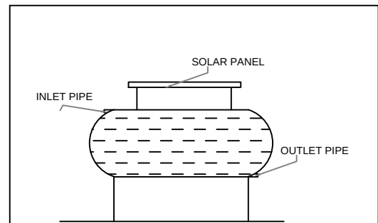
SOLAR SYSTEM
