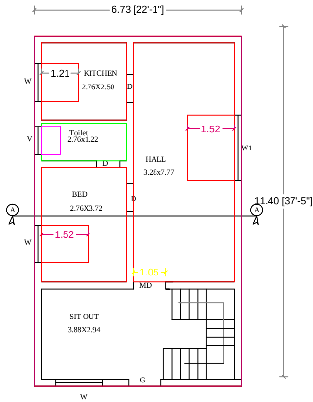
PLAN
