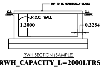
RWH_CAPACITY_L=2000LTRS
