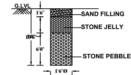
RAIN WATER HARVESTING PIT (NOT TO SCALE)
