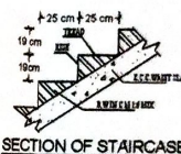
SECTION OF STAIRCASE
