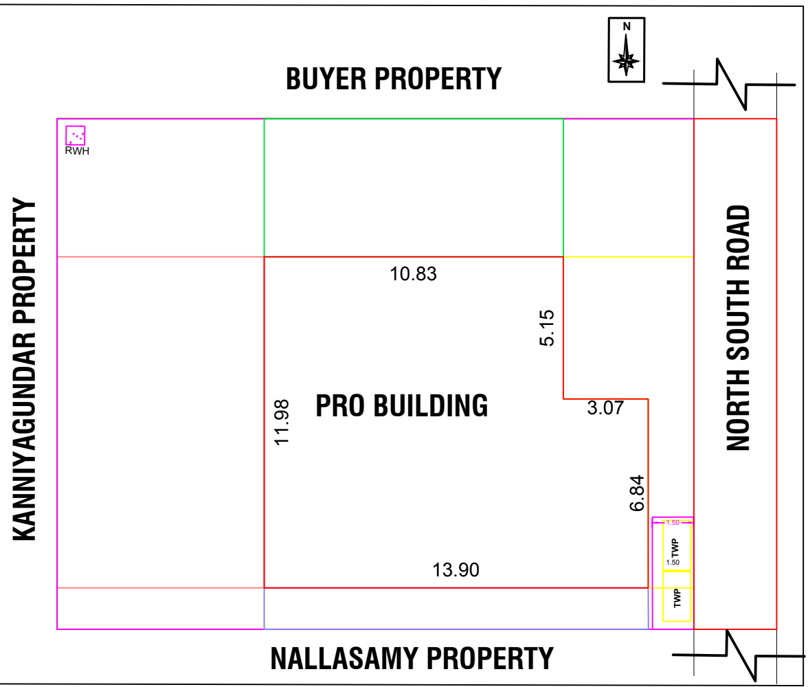
SITE PLAN
