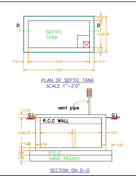
SECTION ON D-D
