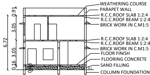
SECTION- SS
