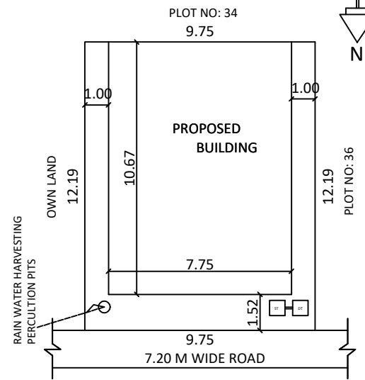
SITE PLAN
