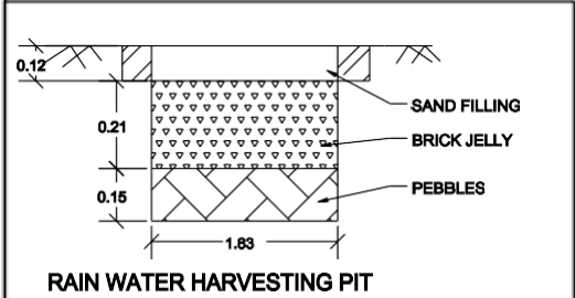
RAIN WATER HARVESTING PIT
