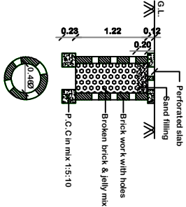
PERCOLATION PIT FOR 30 Sq. m. (Scale:- 1:50)
