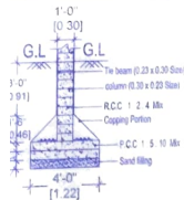
SECTION-IT
