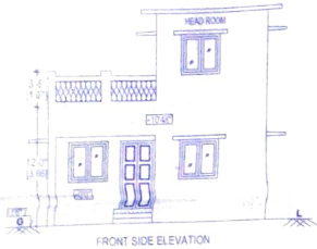
FRONT SIDE ELEVATION
