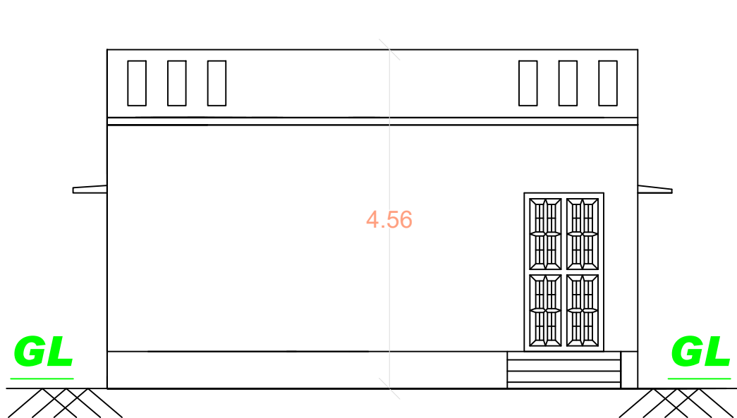
FRONT ELEVATION
