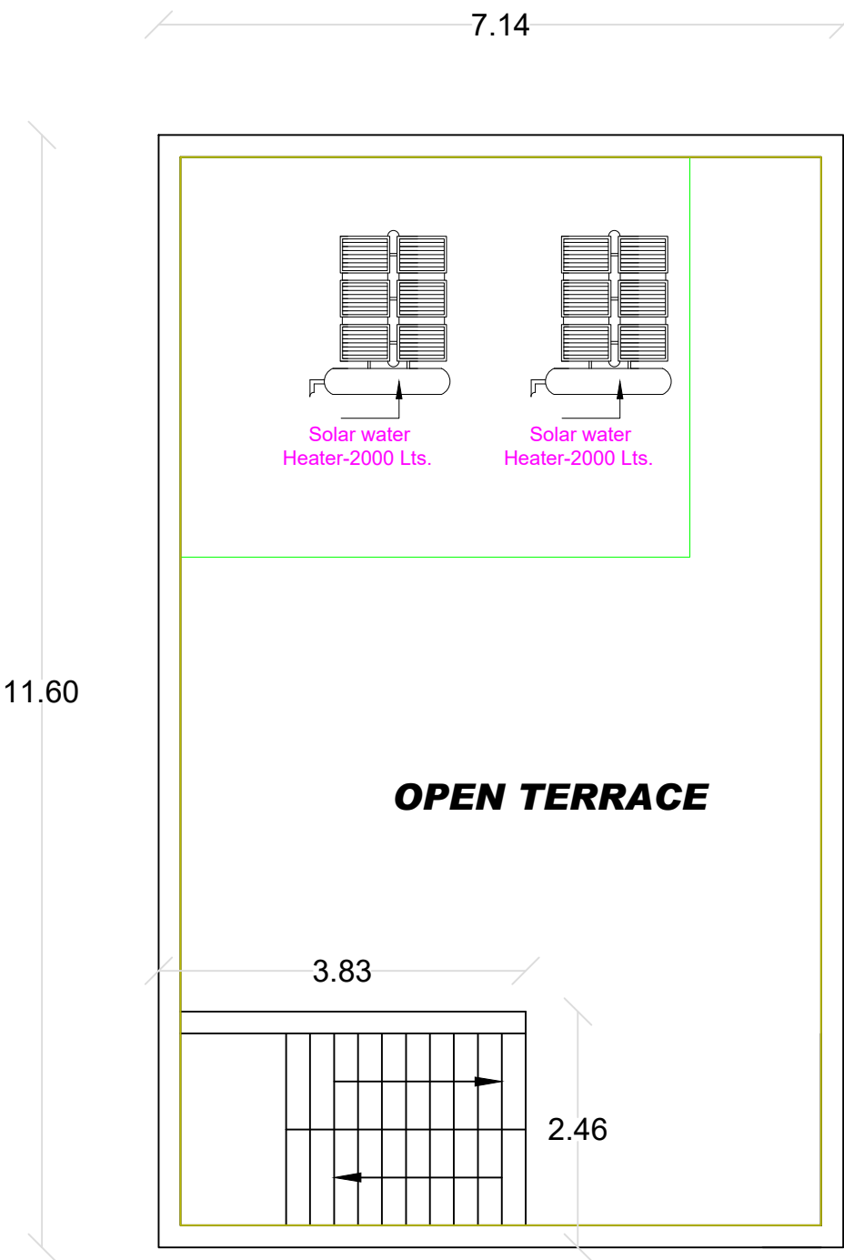
OPEN TERRACE PLAN
