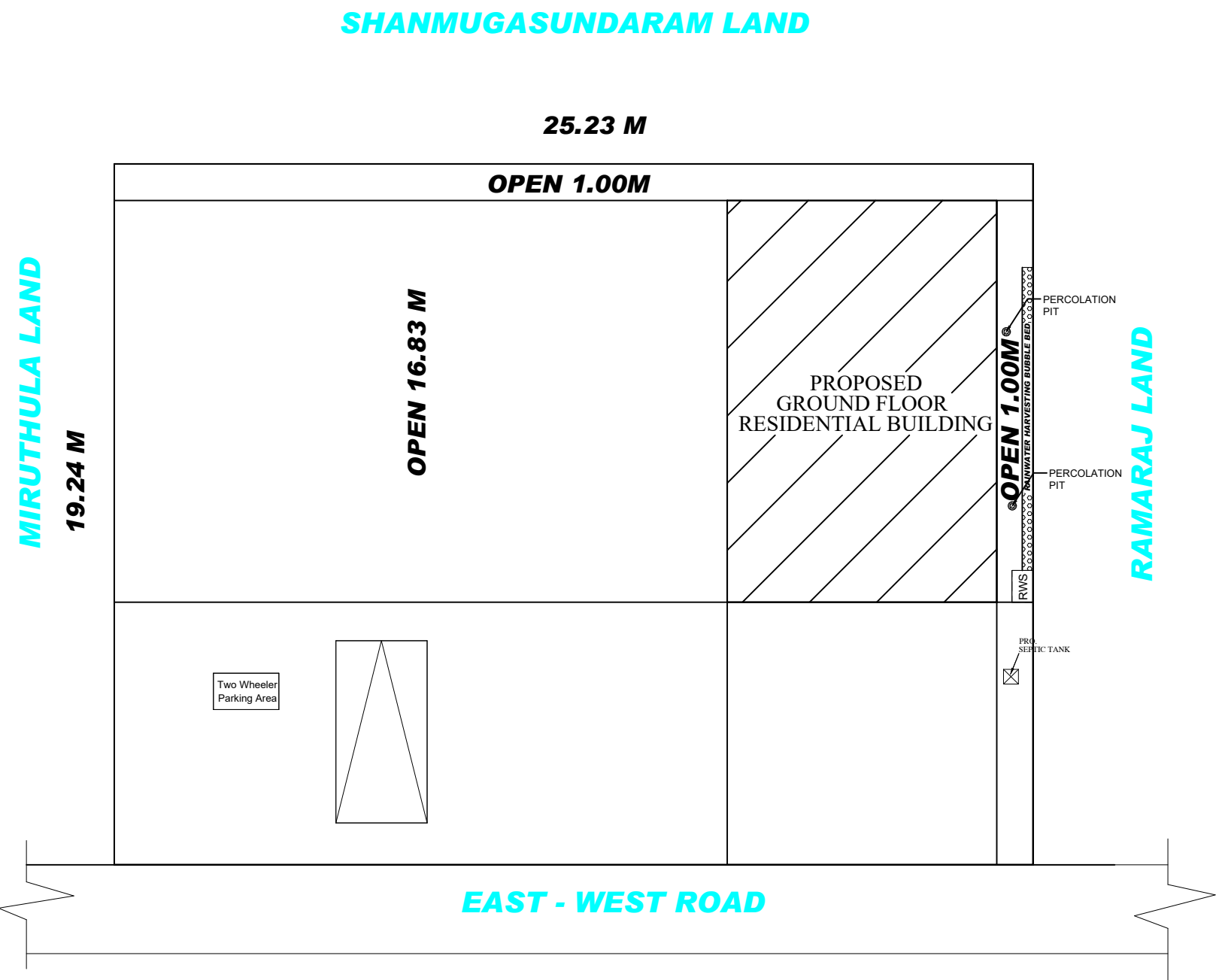
SITE PLAN
