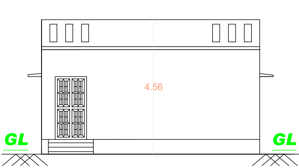
FRONT ELEVATION
