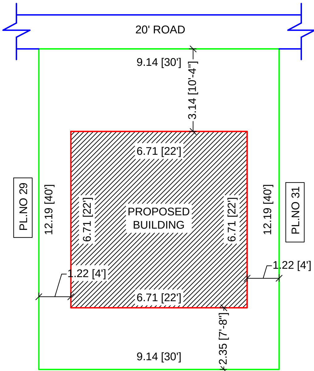
SITE PLAN (1:100)
