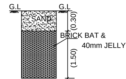
RAIN WATER HARVESTING SYSTEM
