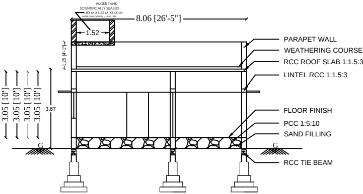
SECTION ON BB
