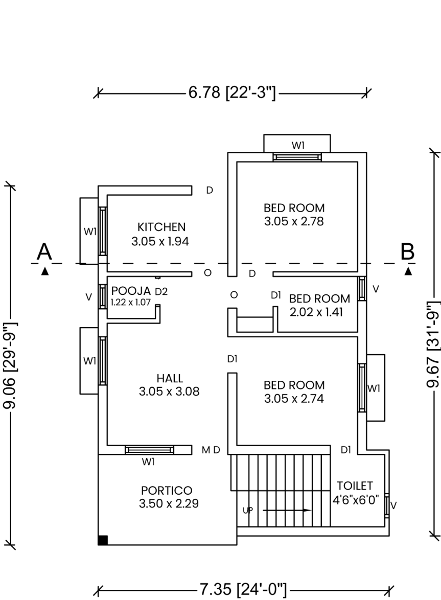
PLAN
