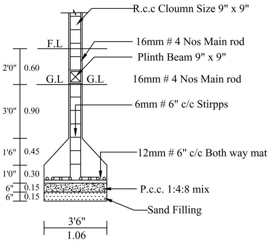
COLUMN DETIALS
