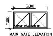
MAIN GATE ELEVATION
