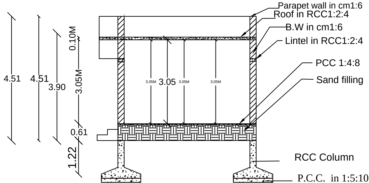
SECTION PLAN
