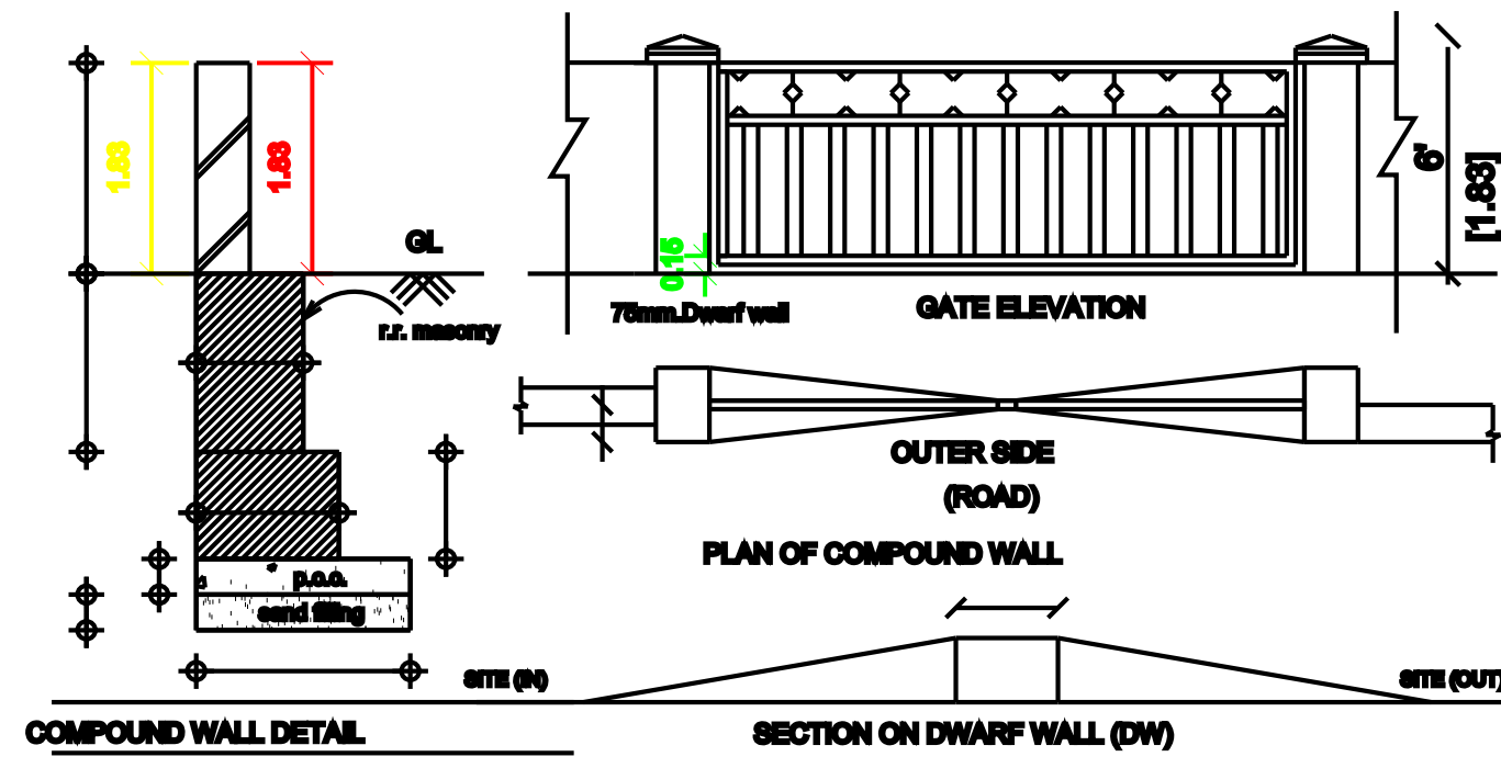
PLAN OF COMPOUND WALL
