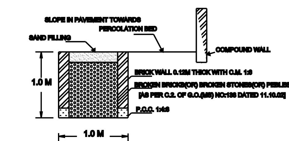
SECTION OF RAIN WATER PERCOLATION BED
