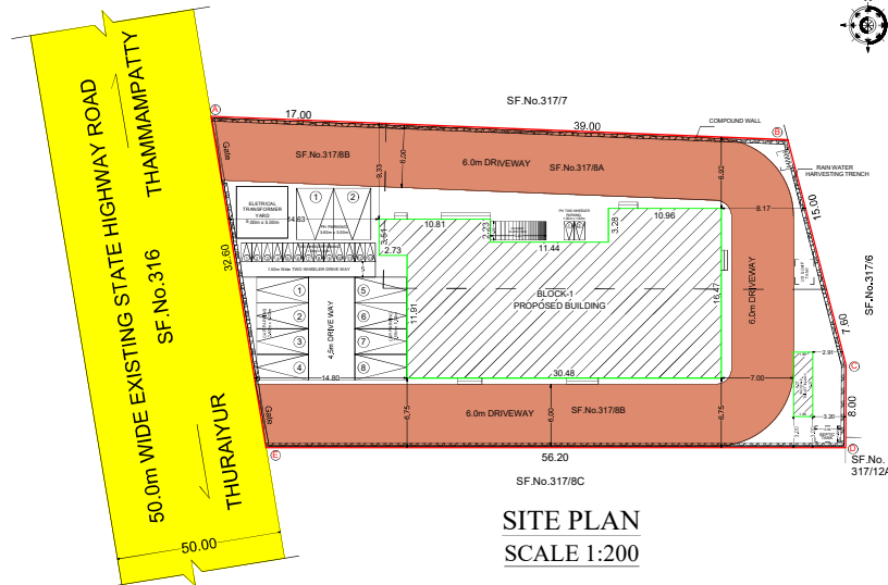
KALYANA MANDAPAM BLOCK -1
