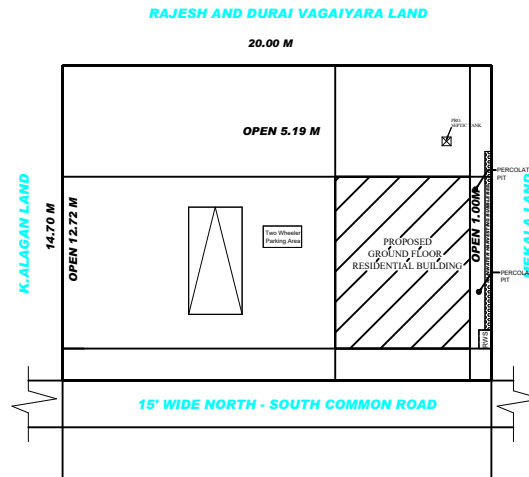
SITE PLAN (SCALE 1:1)
