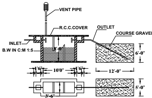
SEPTIC TANK & D-TRENCH DETAILS (NOT TO SCALE)
