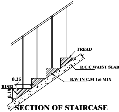
SECTION OF STAIRCASE (NOT TO SCALE)
