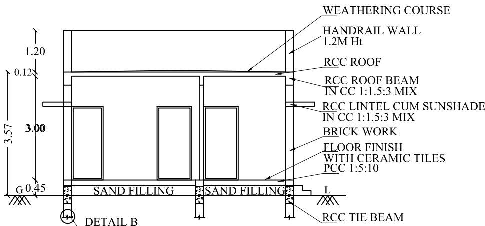
SECTION AB
