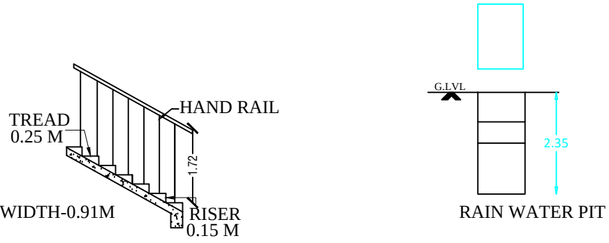
STAIRCASE DETAILS
