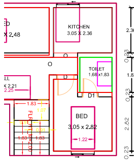
1. FIRST FLOOR PLAN.
