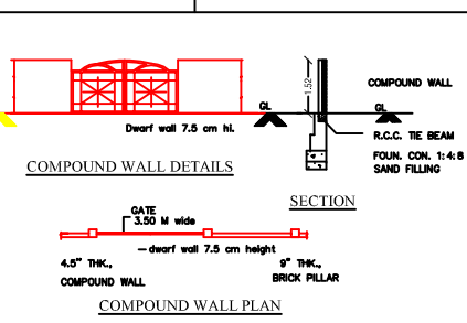
COMPOUND WALL DETAILS
