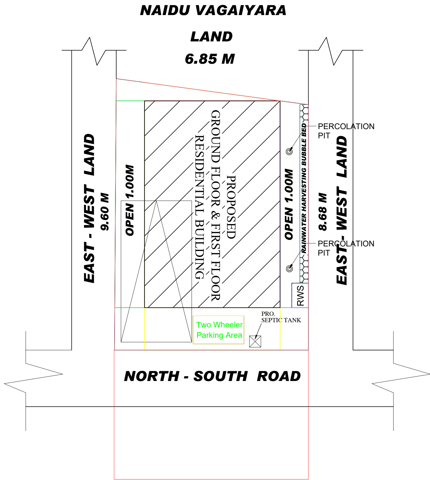
SITE PLAN (SCALE 1:1)
