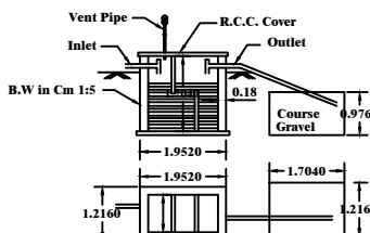
SEPTIC TANK & D-TRENCH DETAILS
