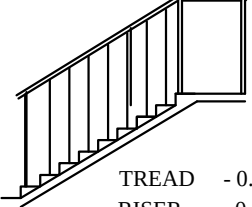
STAIRCASE DETAILS
