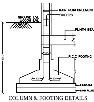
COLUMN & FOOTING DETAILS
