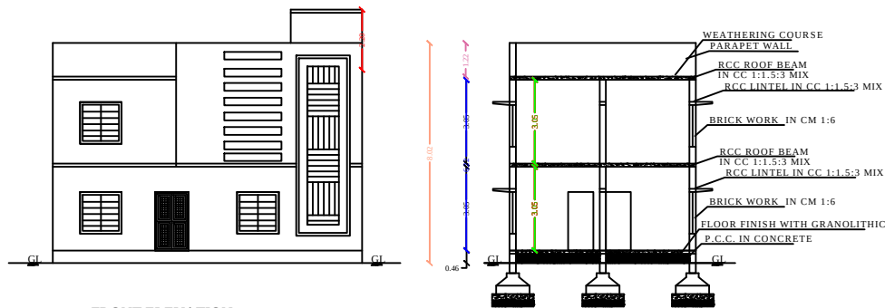
FRONT ELEVATION
