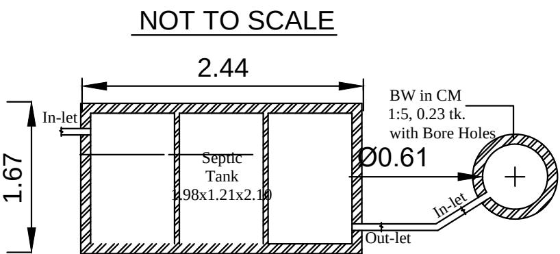
PLAN - SEPTIC TANK & SOAK PIT
