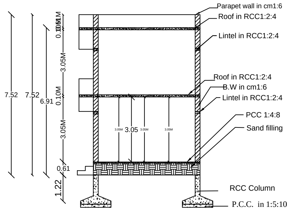
SECTION PLAN
