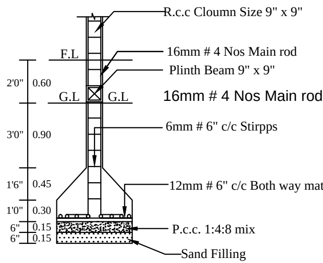
COLUMN DETIAL
