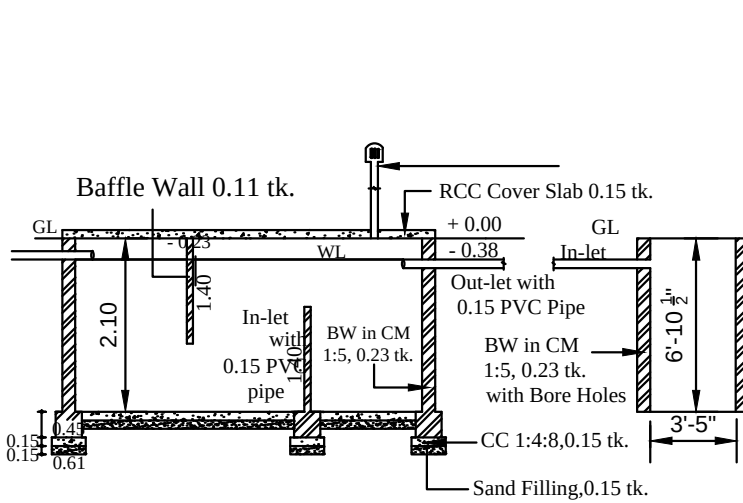
SECTION - SEPTIC TANK & SOAK PIT
