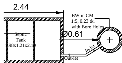
SEPTIC TANK & SOAK PIT
