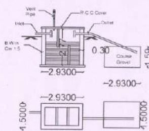
SEPTIC TANK & D-TRENCH DETAILS
