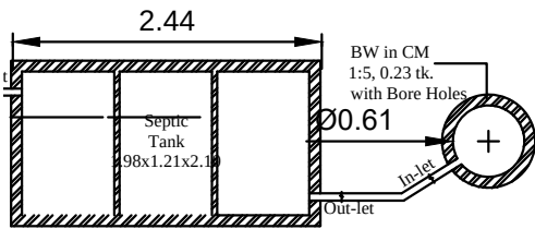
PLAN - SEPTIC TANK & SOAK PIT
