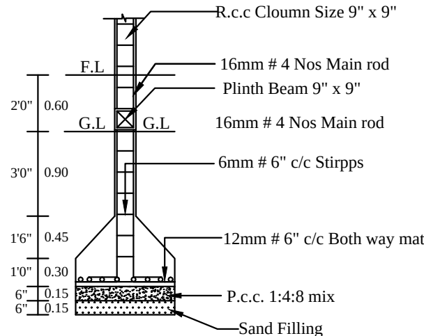
COLUMN DETIAL
