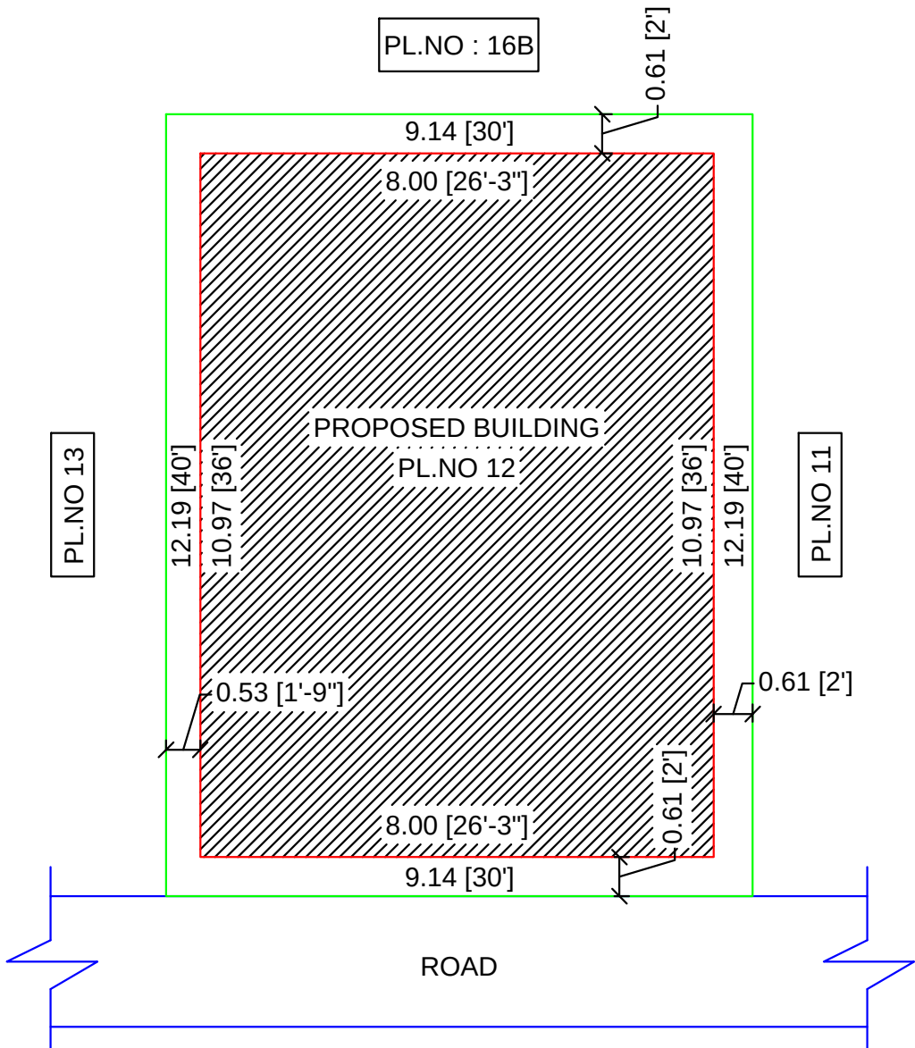
SITE PLAN (1:100)
