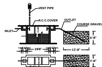
SEPTIC TANK & D-TRENCH DETAILS (NOT TO SCALE)
