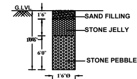
RAIN WATER HARVESTING PIT (NOT TO SCALE)
