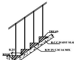
SECTION OF STAIRCASE (NOT TO SCALE)
