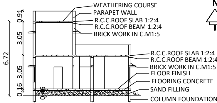
SECTION- SS
