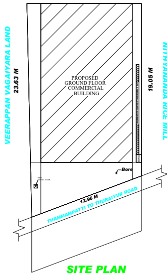
SITE PLAN
